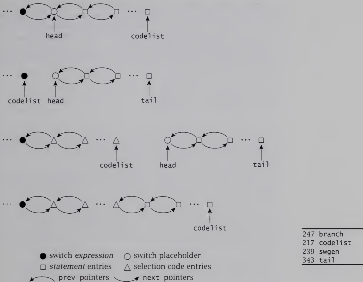
FIGURE 10.2 Code-list manipulations for generating switch selection code.
