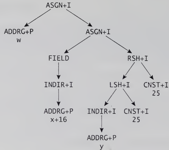
FIGURE 12.5 Tree for w = x.amt = y .
