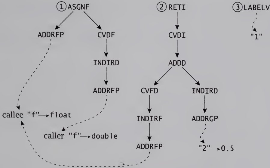
FIGURE 1.3 Dags for the sample.
