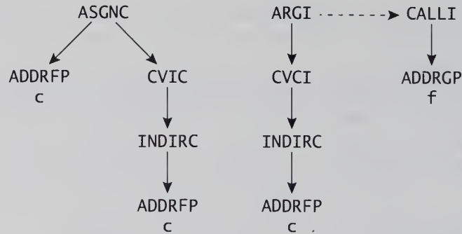
FIGURE 5.2 Forests for f(char c) { f(c); }
