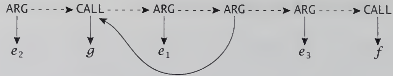
FIGURE 12.10 Forest for f(e_1, g(e_2), e_3) .
