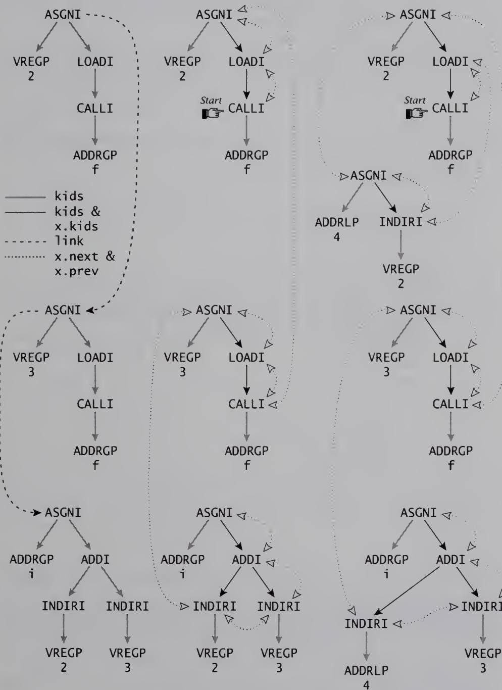
FIGURE 15.3 Spilling in i = f() + f() .
