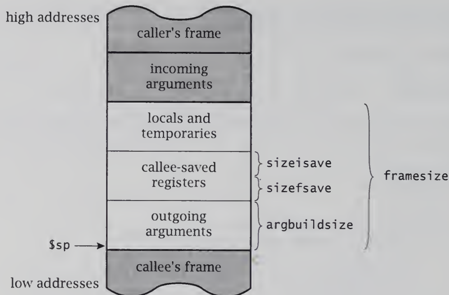
FIGURE 16.1 MIPS stack frame.
