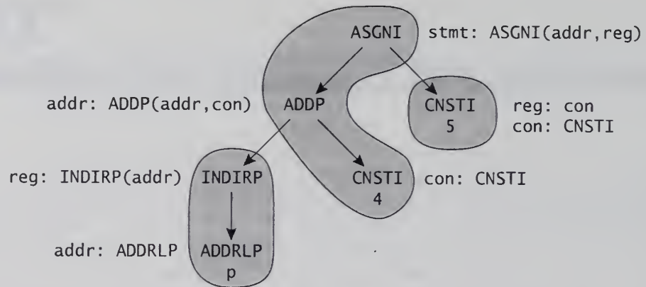
FIGURE 14.1 Cover for \text{ASGNI}(\text{ADDP}(\text{INDIRP}(\text{ADDRLP}(p)), \text{CNSTI}(4)), \text{CNSTI}(5)) .
