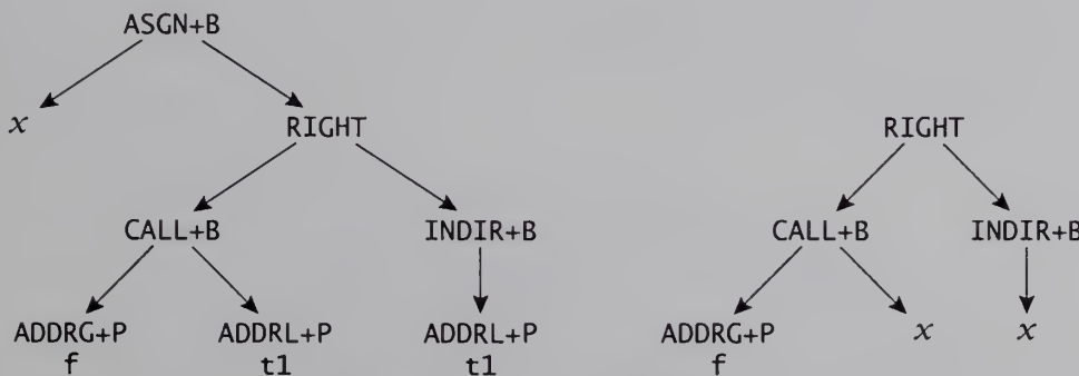
FIGURE 9.5 Trees for x=f() .
