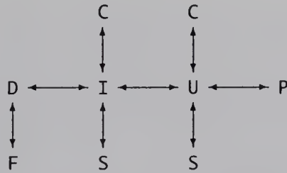
FIGURE 9.1 Conversions.
