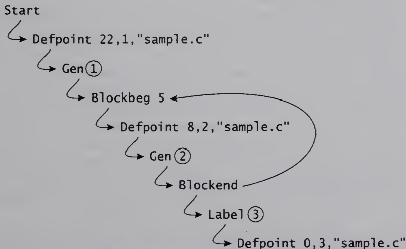
FIGURE 1.4 Code list for the sample.
