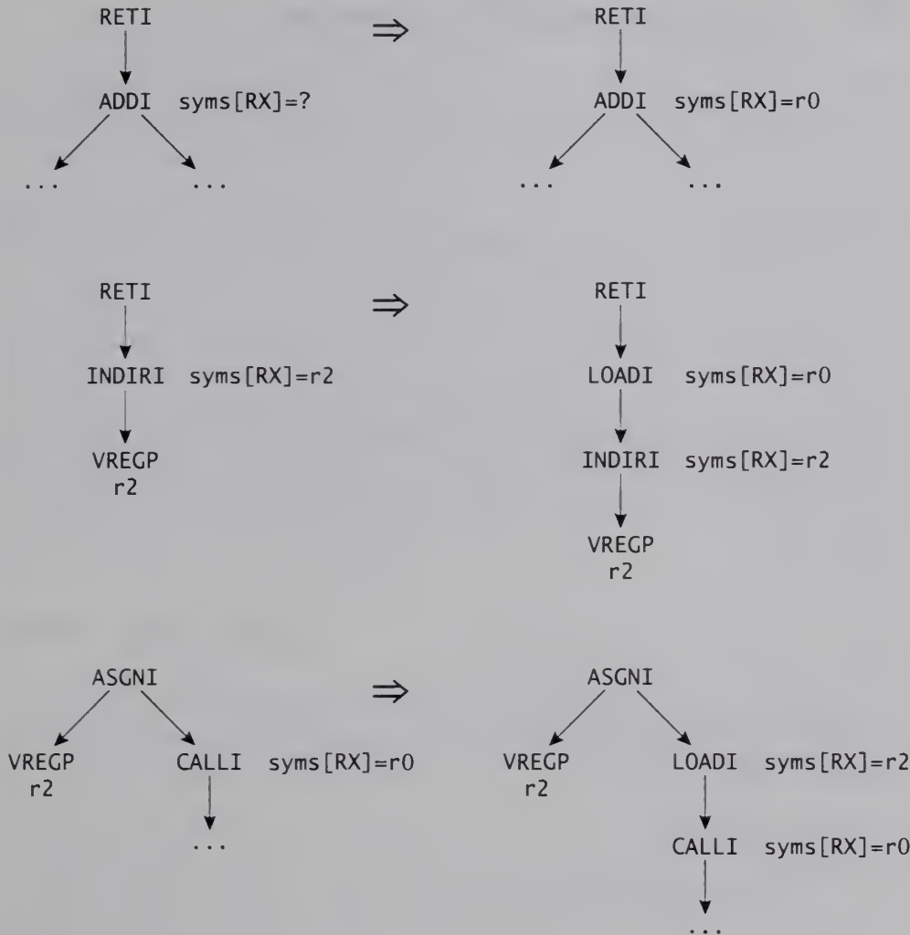
FIGURE 14.6 rtarget samples.
