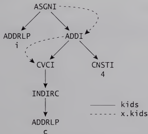
FIGURE 14.5 Figure 14.3 pruned.
