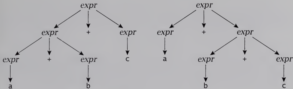
FIGURE 7.1 Two parse trees for a+b+c .
