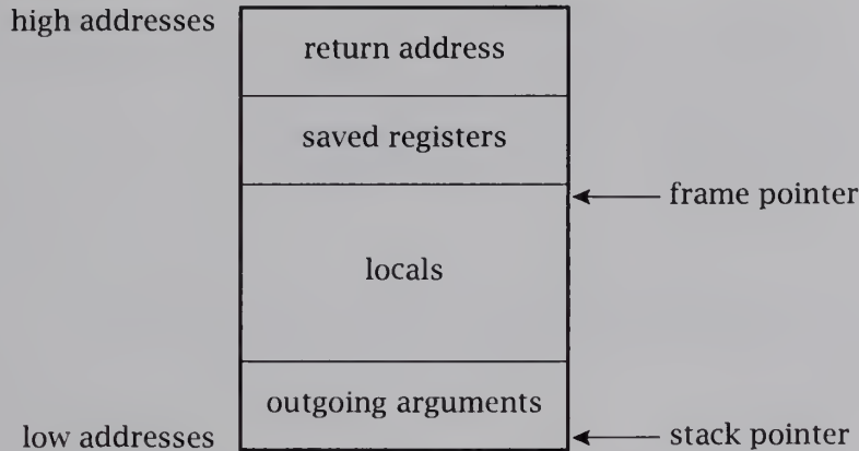
FIGURE 13.3 Typical frame.
