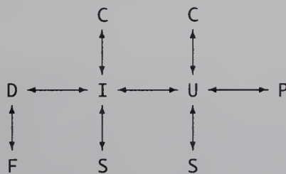
FIGURE 5.1 Conversions.
