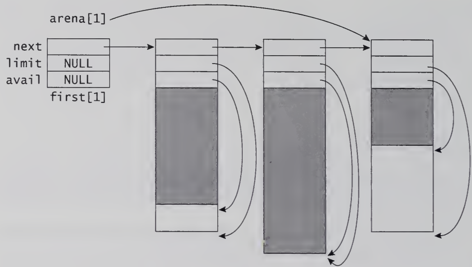
FIGURE 2.1 Arena representation.
