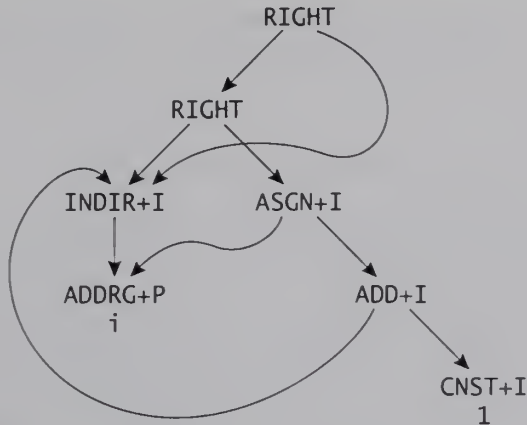
FIGURE 12.11 Tree for i++ .
