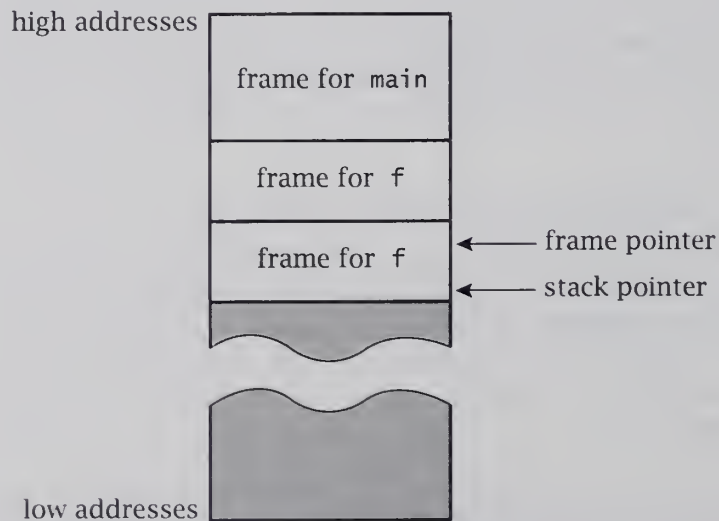
FIGURE 13.2 Three stack frames.
