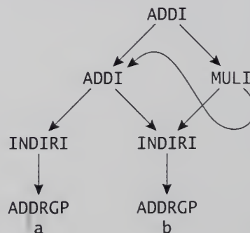
FIGURE 12.1 Dag for (a+b)+b*(a+b) .
