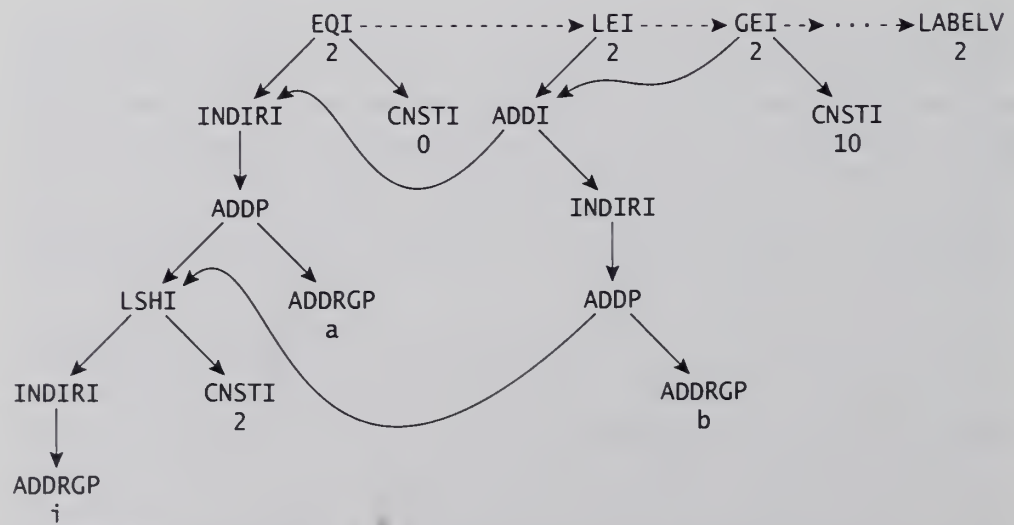
FIGURE 12.3 Forest for a[i] \ \&\& \ a[i]+b[i] > 0 \ \&\& \ a[i]+b[i] < 10 .
