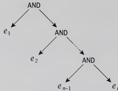
FIGURE 12.2 Tree for e_1 \ \&\& \ e_2 \ \&\& \ \dots \ \&\& \ e_n .
