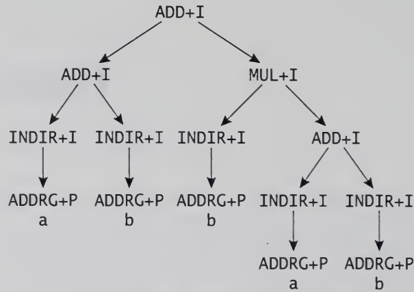
FIGURE 8.1 Abstract syntax tree for (a+b)+b*(a+b) .
