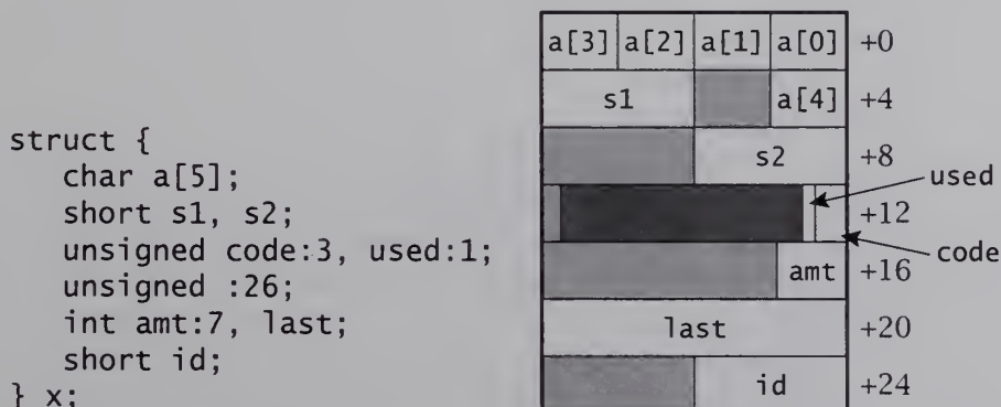
FIGURE 11.1 Little-endian structure layout example.
