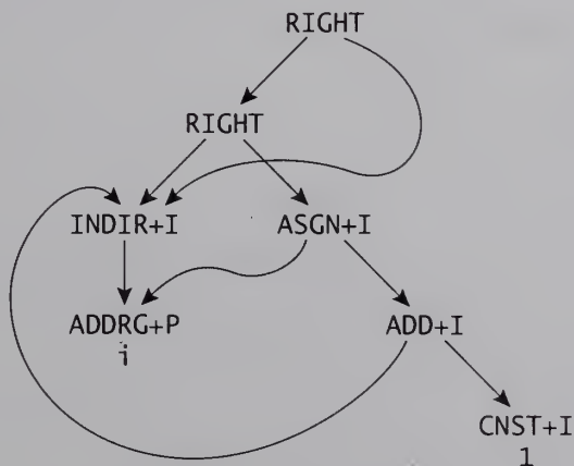
FIGURE 8.3 Tree for i++ .
