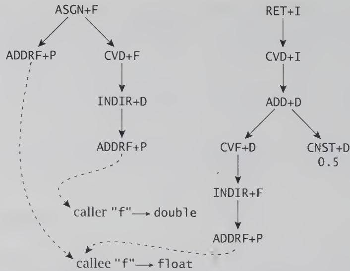
FIGURE 1.2 Abstract syntax trees for the sample.
