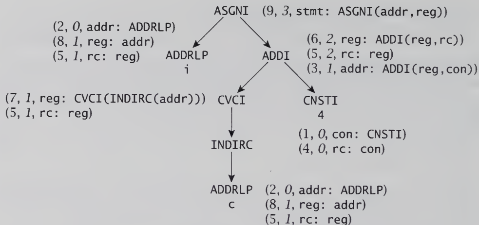
FIGURE 14.3 Labelled tree for i = c + 4 .
