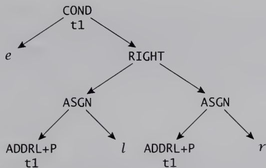
FIGURE 12.4 Tree for e ? l : r .
