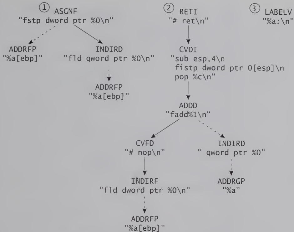
FIGURE 1.5 After selecting instructions.
