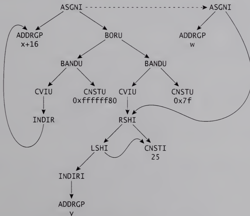
FIGURE 12.6 Forest for w = x.amt = y .
