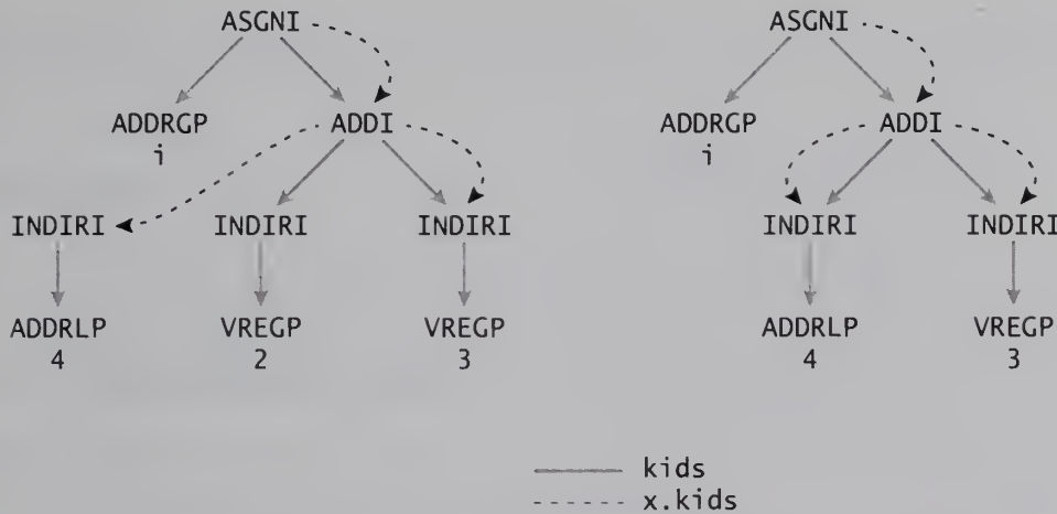
FIGURE 15.4 Figure 15.3's reload before and after re prune.
