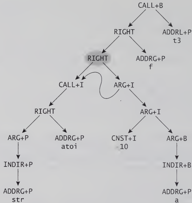
FIGURE 9.2 Tree for f(a, '\n', \text{atoi}(\text{str})) .
