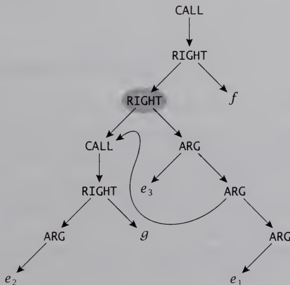
FIGURE 12.9 Tree for f(e_1, g(e_2), e_3) .
