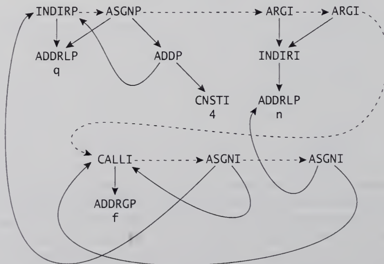
FIGURE 12.12 Forest for n = *q++ = f(n, n) .
