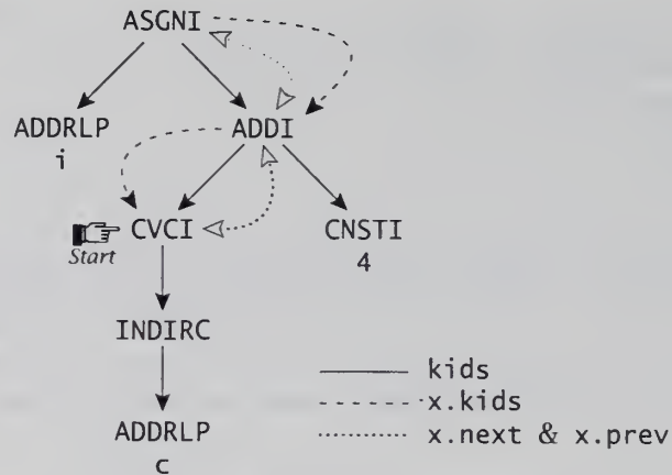
FIGURE 15.1 Ordering uses.
