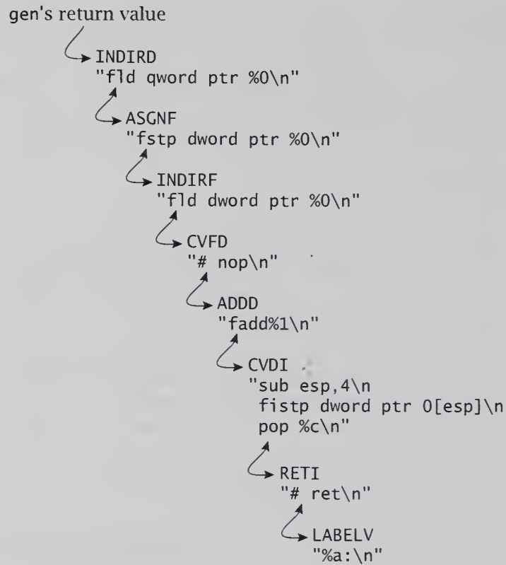
FIGURE 13.1 Figure 1.5 linearized.
