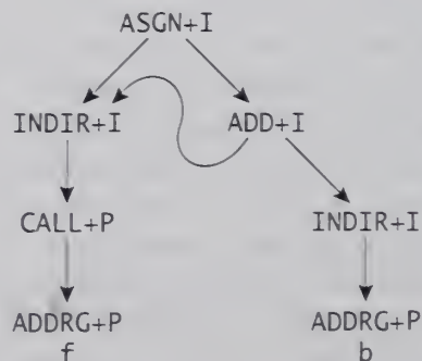
FIGURE 8.2 Tree for *f() += b .
