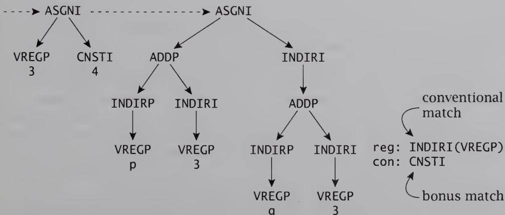
FIGURE 14.4 Excessive common subexpression elimination in p->b=q->b .
