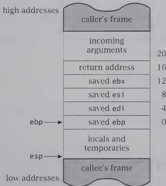
FIGURE 18.1 A frame for the X86.
