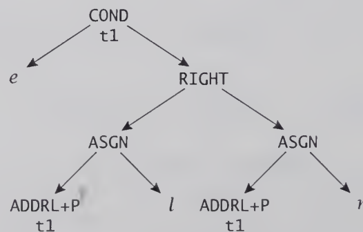
FIGURE 9.6 Tree for e ? l : r .
